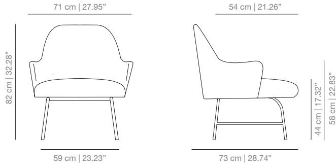
ALBUMEBR metal base lounge chair with armrest
