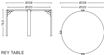
REY TABLE DIAMETER 128 CM | 50.4" DIAMETER TABLETOP 120 CM | 47.24" HEIGHT 74,5 CM | 29.33"
