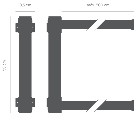
DUAL wall
