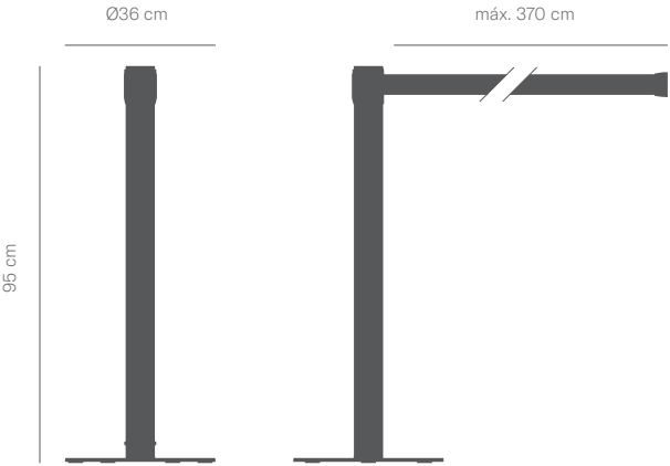
ECO Post Esc. 1:20 (Weight: 8kg) Ref: D/LI/ PE / * (color)
