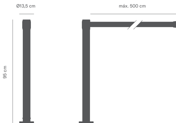
FIX Post
