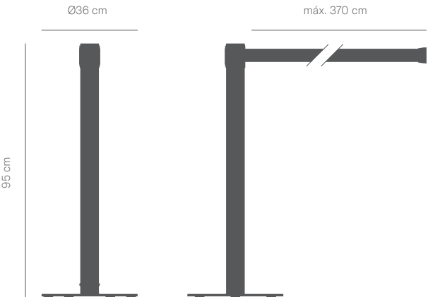
LIMIT Post Esc. 1:20 (Weight: 11kg) Ref: D/LI/ P / * (color)
