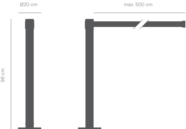
MAG Post Esc. 1:20 (Weight: 4kg) Ref: D/LI/ PMG / * (color)
