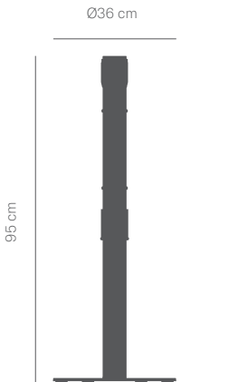
LIMIT DUAL Post Esc. 1:20 (Weight: 11Kg) D/LI/ PDUA
