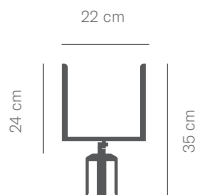
Notice holder BASIC A4 V Esc. 1:20 (Weight: 0,7kg) D/LI/ PCB/A4V
