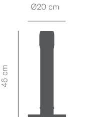
MAG MINI Post Esc. 1:20 (Weight: 3kg) D/LI/ PMI
