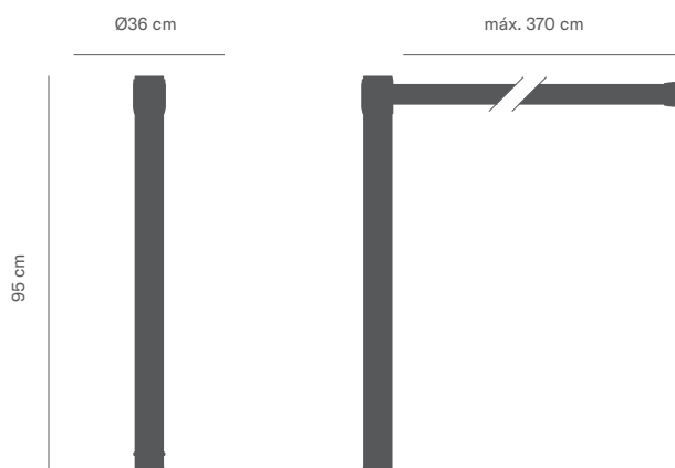
ECO Post
