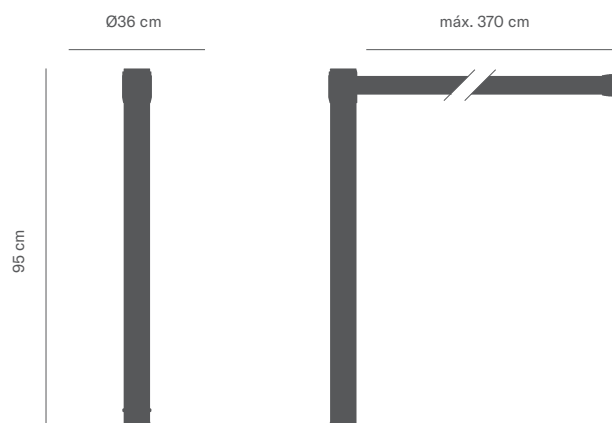
LIMIT Post
