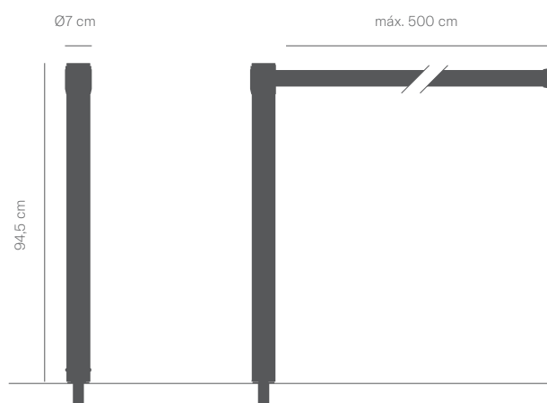
UNFIX Post
