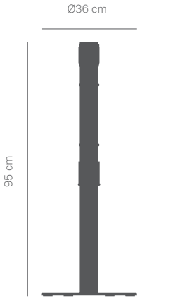
ECO DUAL Post Esc. 1:20 (Weight: 8Kg) D/LI/ PDUA
