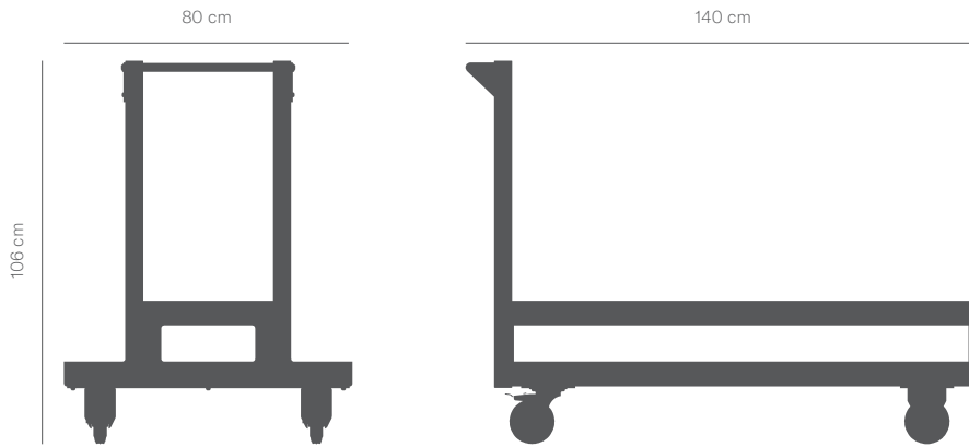
TROLLEY Esc. 1:20 (Weight: 40kg) Ref: D/ CAR
