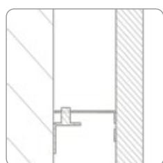
WALL SUSPENSION
