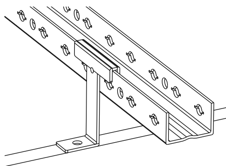
U-PROFILE SUSPENSION
