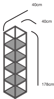
Floorstanding Colourframe (5 high) Connecting Frame 40cm wide 40cm deep 178cm high
