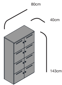
Locker Door Cabinet (8 doors) Soft Close Hinges Plain or post slot Key or combination lock 80cm wide 40cm deep 143cm high
