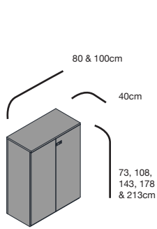
Hinged Door Cabinet 2, 3, 4, 5 & 6 high cabinets Soft Close Hinges 80 & 100cm wide 40cm deep 73, 108, 143, 178 and 213cm high
