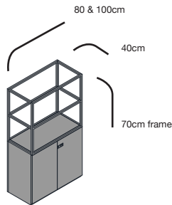
Colourframe (2 high) Seamless welded frame 80 & 100cm wide 40cm deep 70cm high frame
